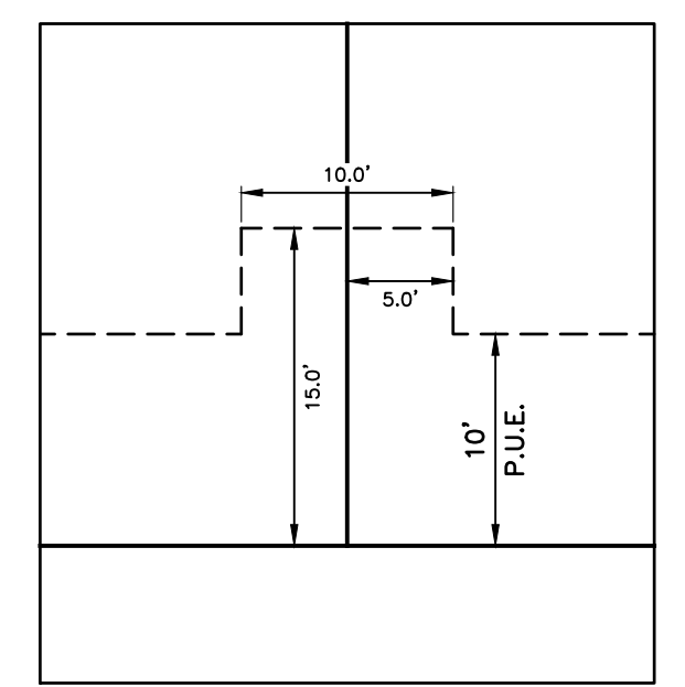
PUBLIC UTILITY EASEMENT DETAIL Scale: 1"=10'
